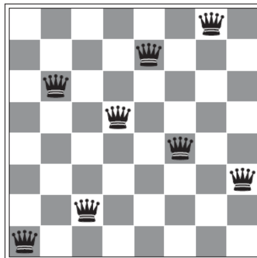
Figure 34 - 8 Queen Problem
