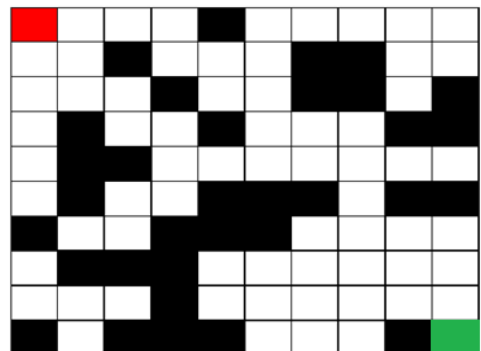
Figure 30 - Maze
